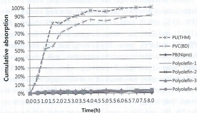
Figure 5. Nitroglycerin absorption behaviors on the inner surface of the different tubes at room temperature.
